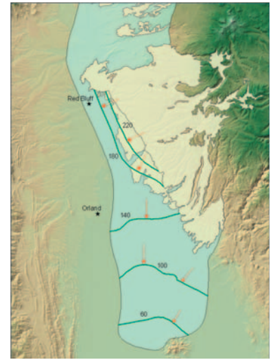
Figure 4. Aerial extent of Tuscan Formation aquifer systems. Light yellow areas show where the upper and lower Tuscan Formations are exposed at ground surface and the blue areas show the approximate buried extents.
