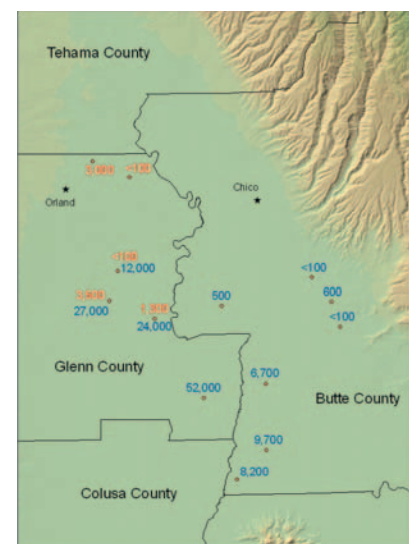
Figure 7. Sample locations and estimated age of the groundwater at various monitoring sites in the north valley. Age is estimated in years; dark blue values represent groundwater in lower Tuscan Formation and red values represent groundwater in Tehama Formation.
