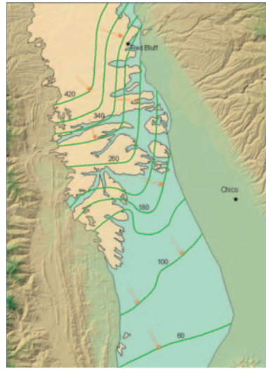
Figure 3. Aerial extent of Tehama Formation aquifer system. Light yellow areas show where the Tehama Formation is exposed at the ground surface and the blue areas show the approximate buried extents.
